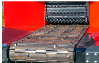
Closed Hardox infeed chain covering the complete length of the infeedtable
